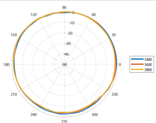
Azimuth: 3400 – 3800 MHz
